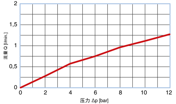
CHECK VALVE® 流量曲线 – screened BFAA055014; T = 50 °C, 液压油 HLP46
