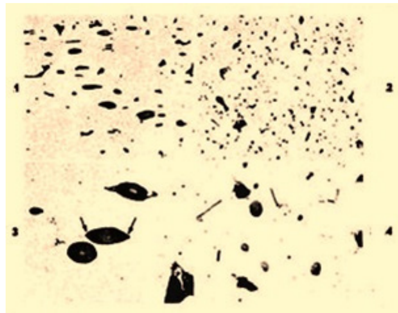
Figure 2: Galena Crystals
